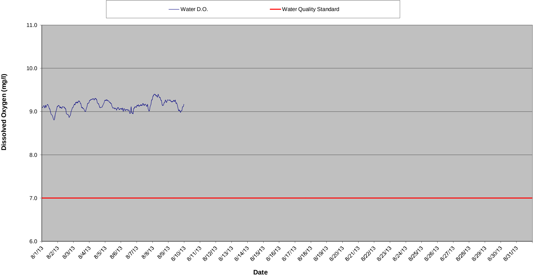
Dead River Below McClure Dam Dissolved Oxygen Summary - August 2013
