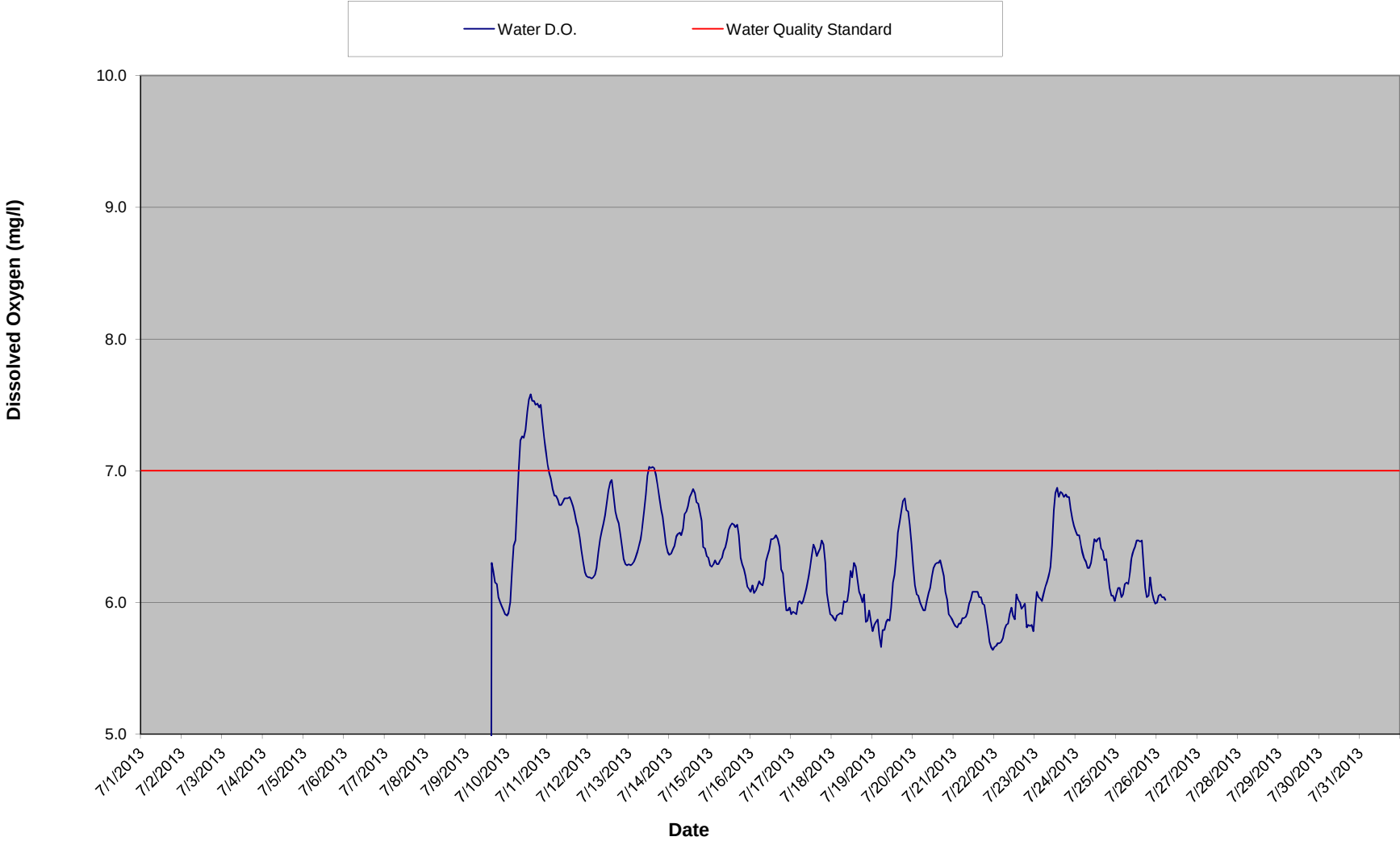
Hoist Powerhouse Dissolved Oxygen Summary - July 2013
