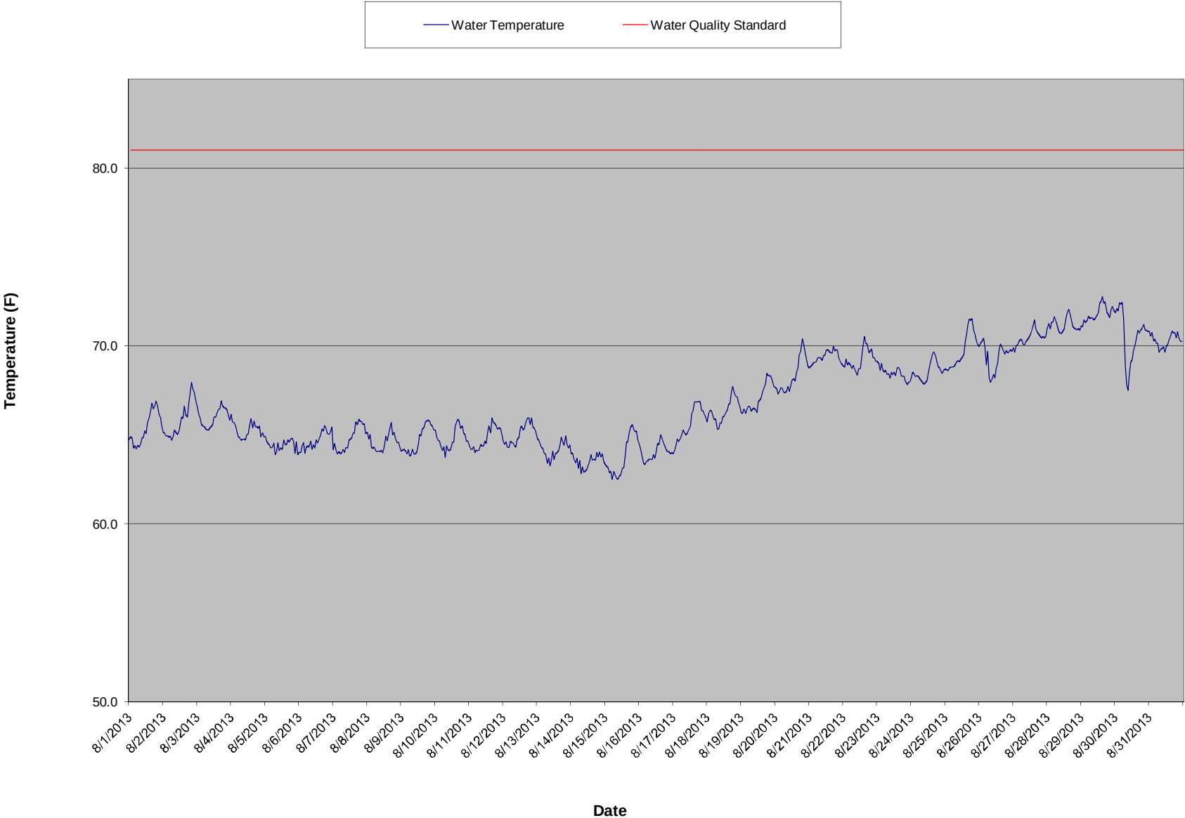
McClure Powerhouse Tailrace Temperature Summary - August 2013
