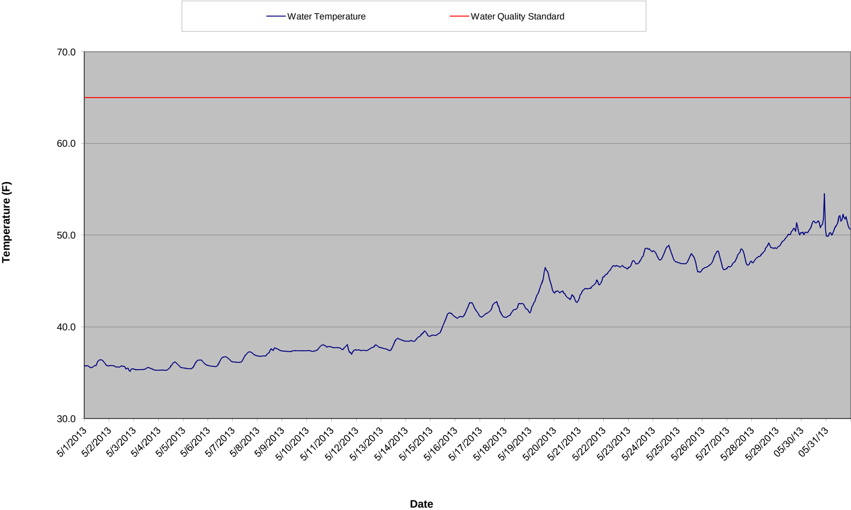
Hoist Powerhouse Temperature Summary - May 2013
