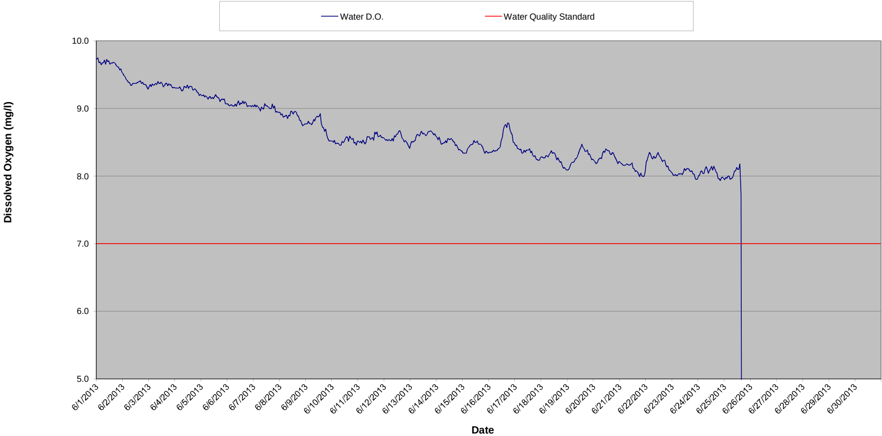
Hoist Powerhouse Dissolved Oxygen Summary - June 2013
