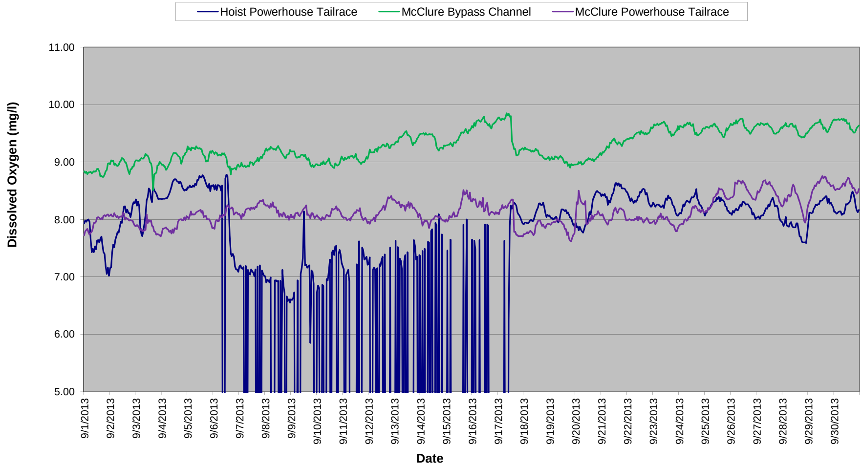
Dissolved Oxygen Comparison - Hoist Powerhouse Tailrace / McClure Bypass Channel / McClure Powerhouse Tailrace - September 2013
