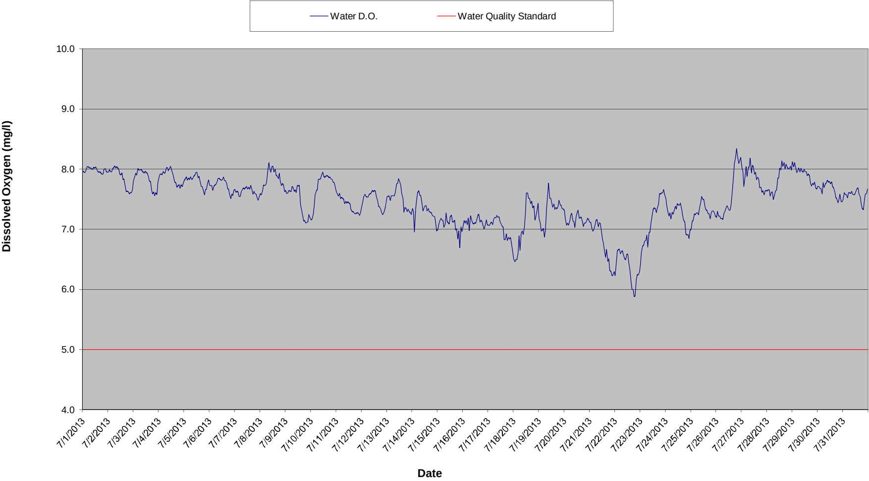
McClure Powerhouse Tailrace DO Summary - July 2013
