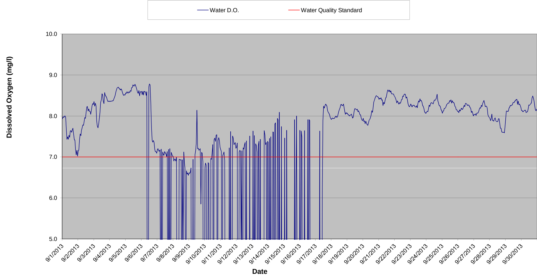
Hoist Powerhouse Dissolved Oxygen Summary - September 2013
