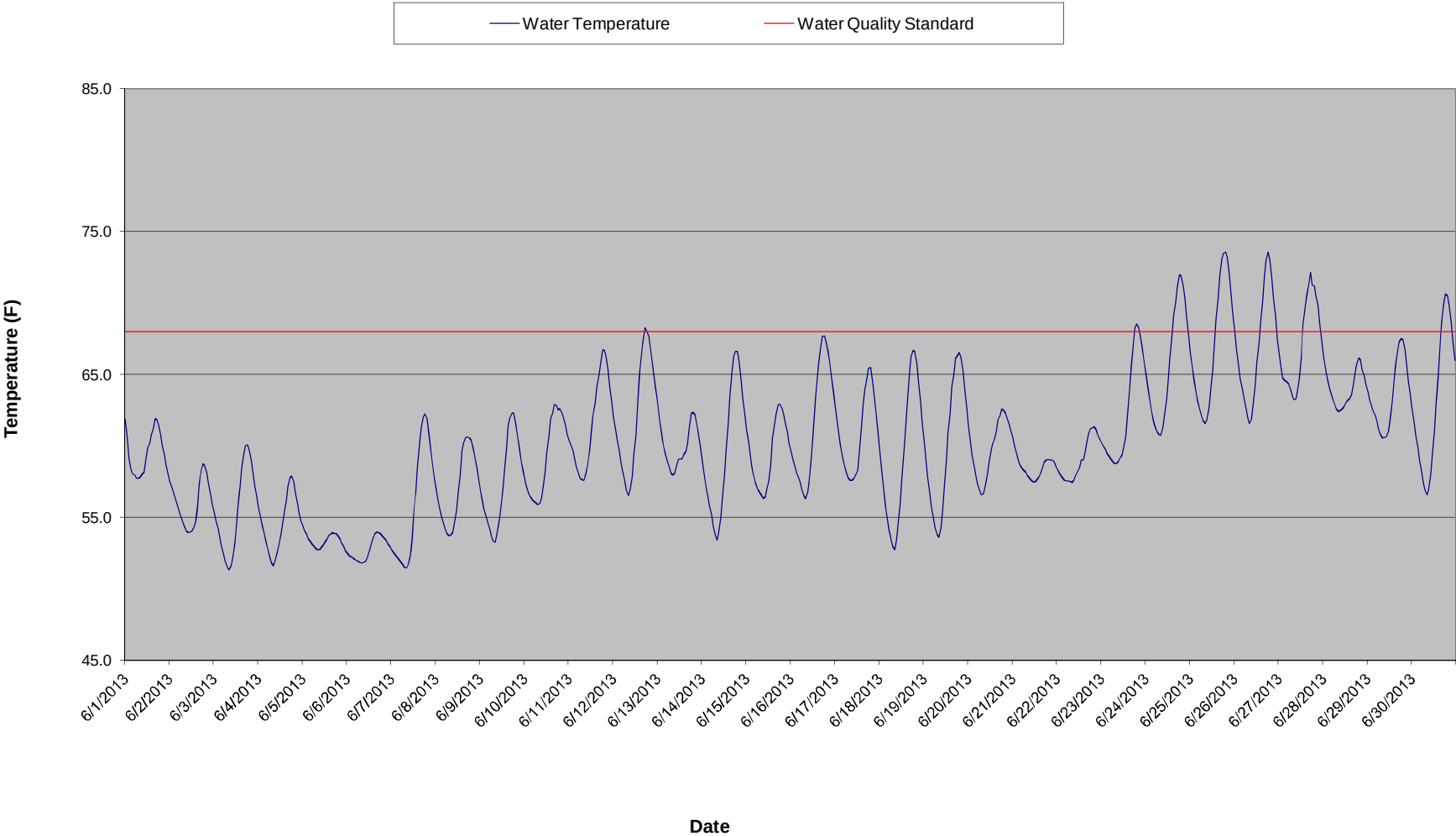
Dead River at CR AAO Bridge Temperature Summary - June 2013
