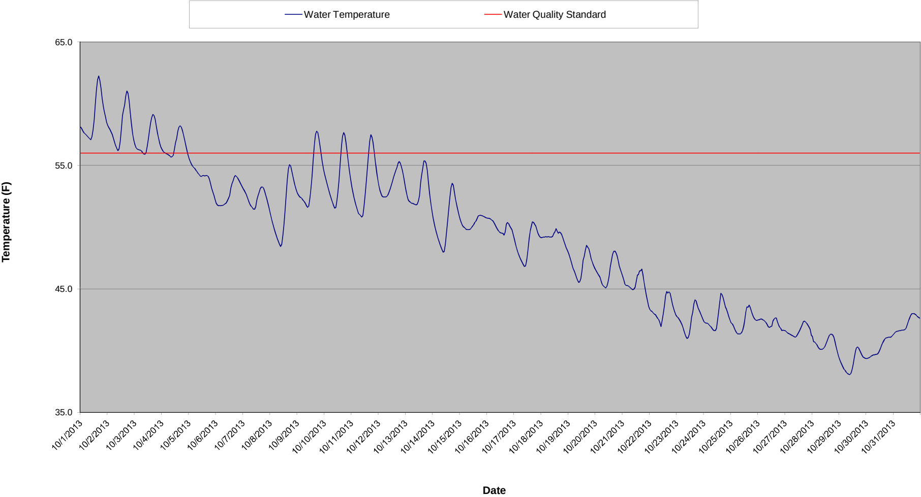
Dead River at CR AAO Bridge Temperature - October 2013
