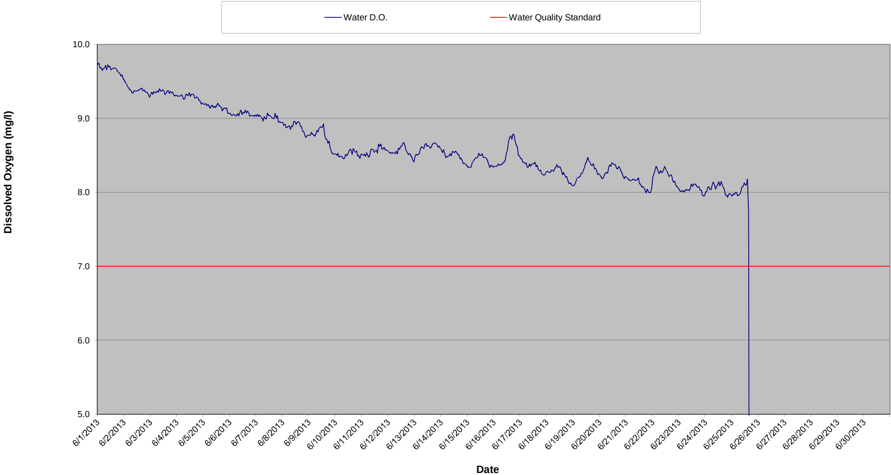
Hoist Powerhouse Dissolved Oxygen Summary - June 2013
