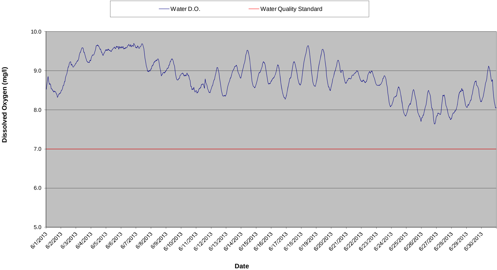
Dead River at CR AAO Bridge Dissolved Oxygen Summary - June 2013
