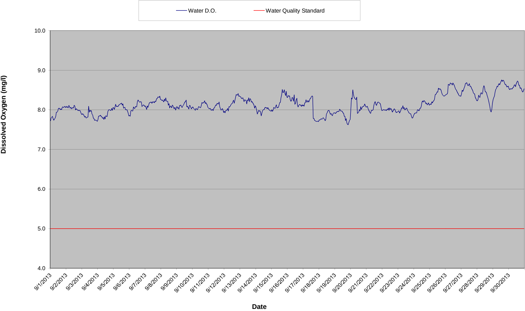
McClure Powerhouse Tailrace DO Summary - September 2013
