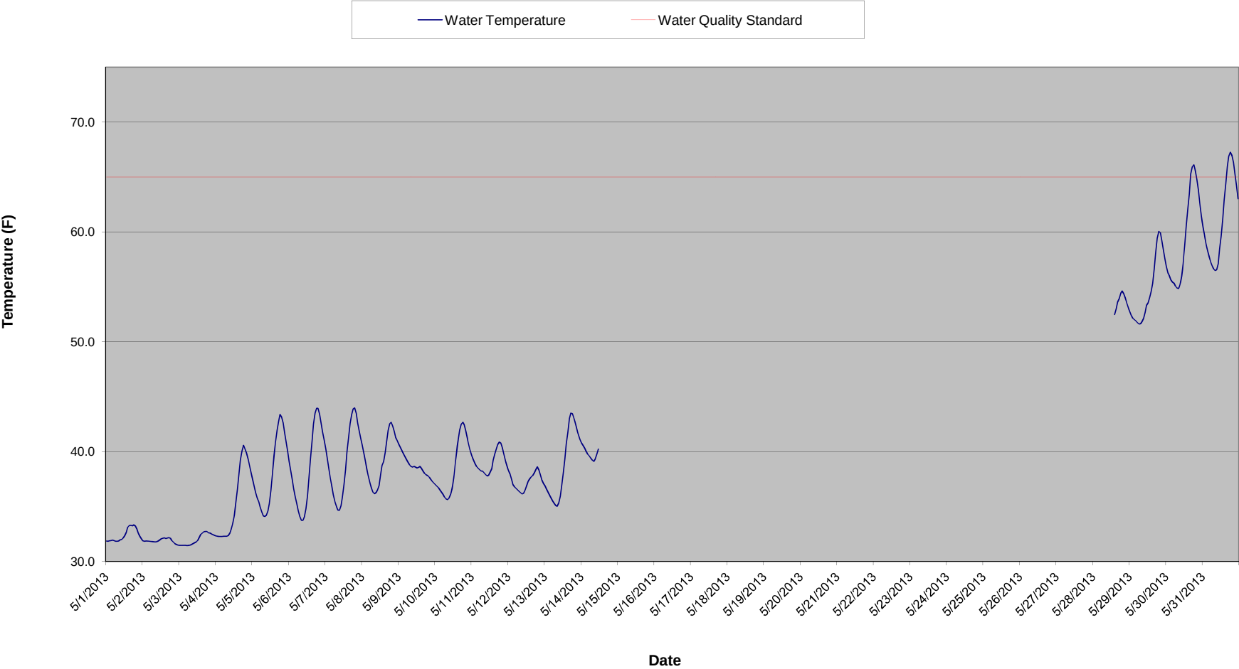
Dead River at CR AAO Bridge Temperature Summary - May 2013
