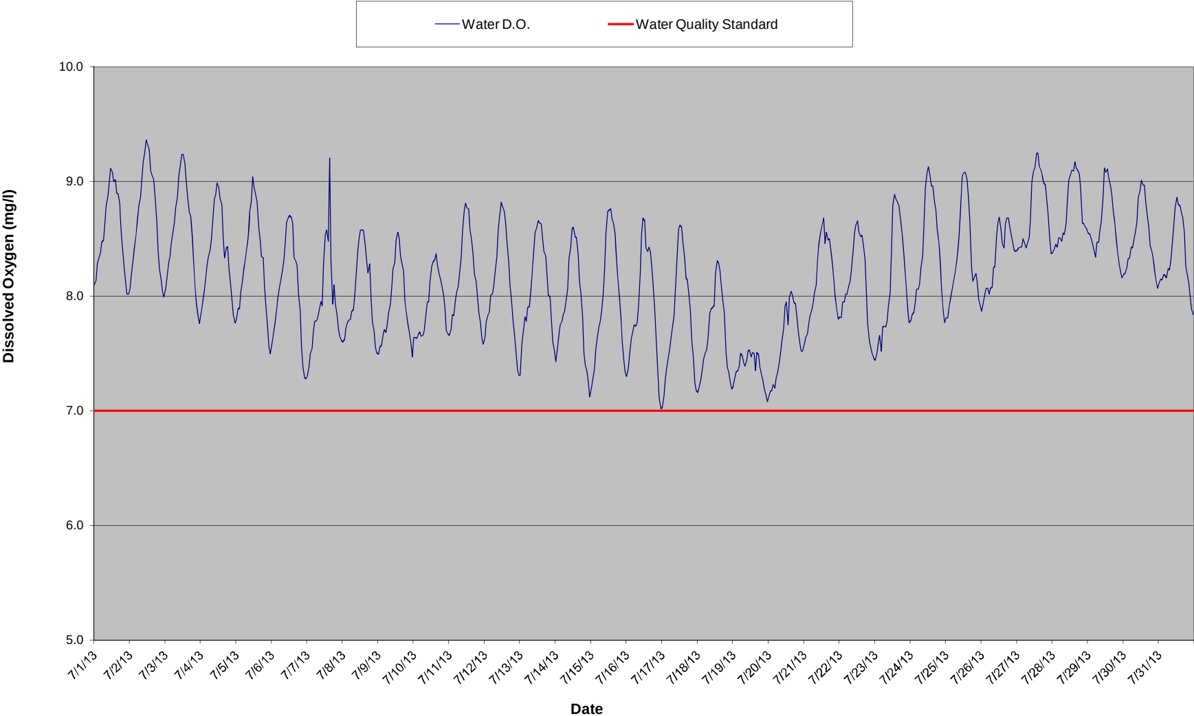
Dead River at CR AAO Bridge Dissolved Oxygen Summary - July 2013
