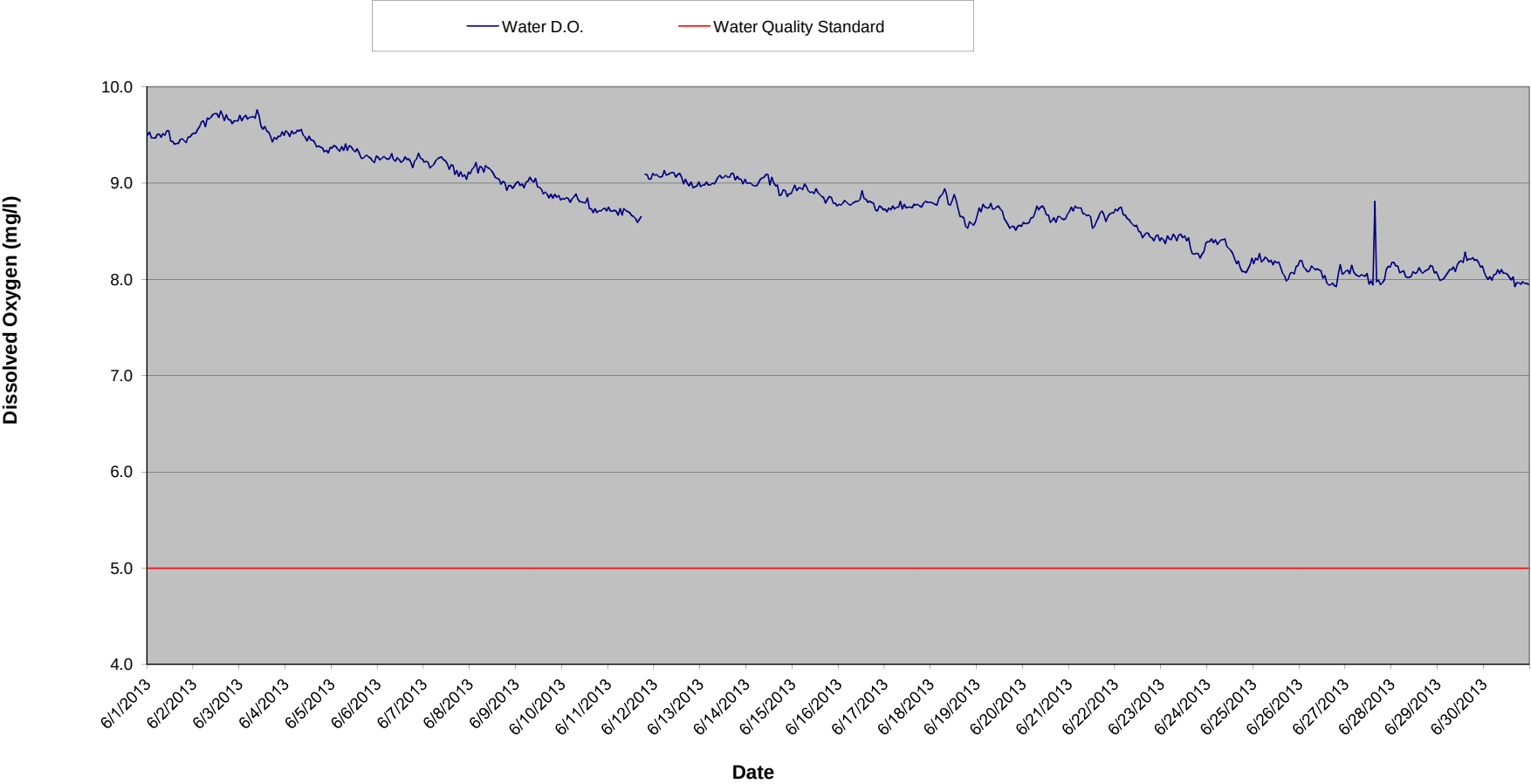
McClure Powerhouse Tailrace DO Summary - June 2013
