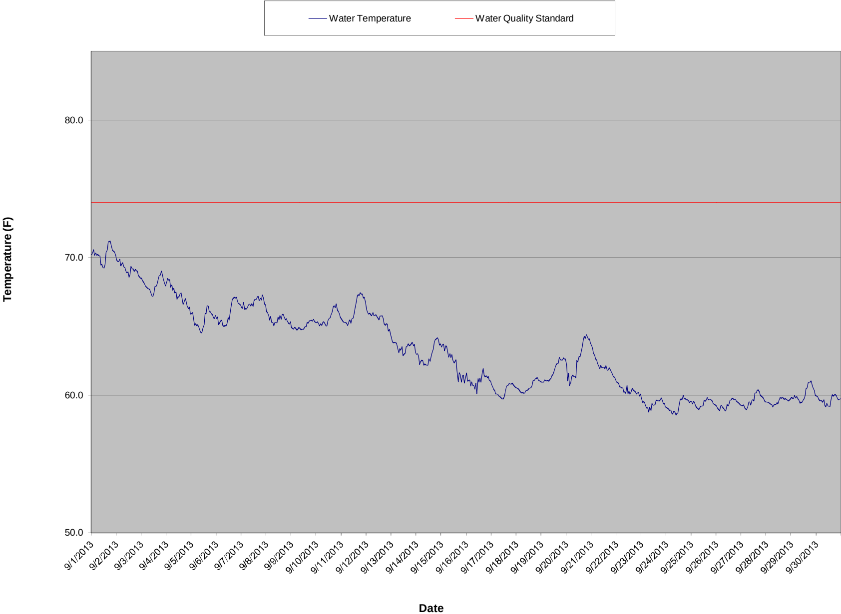
McClure Powerhouse Tailrace Temperature Summary - September 2013
