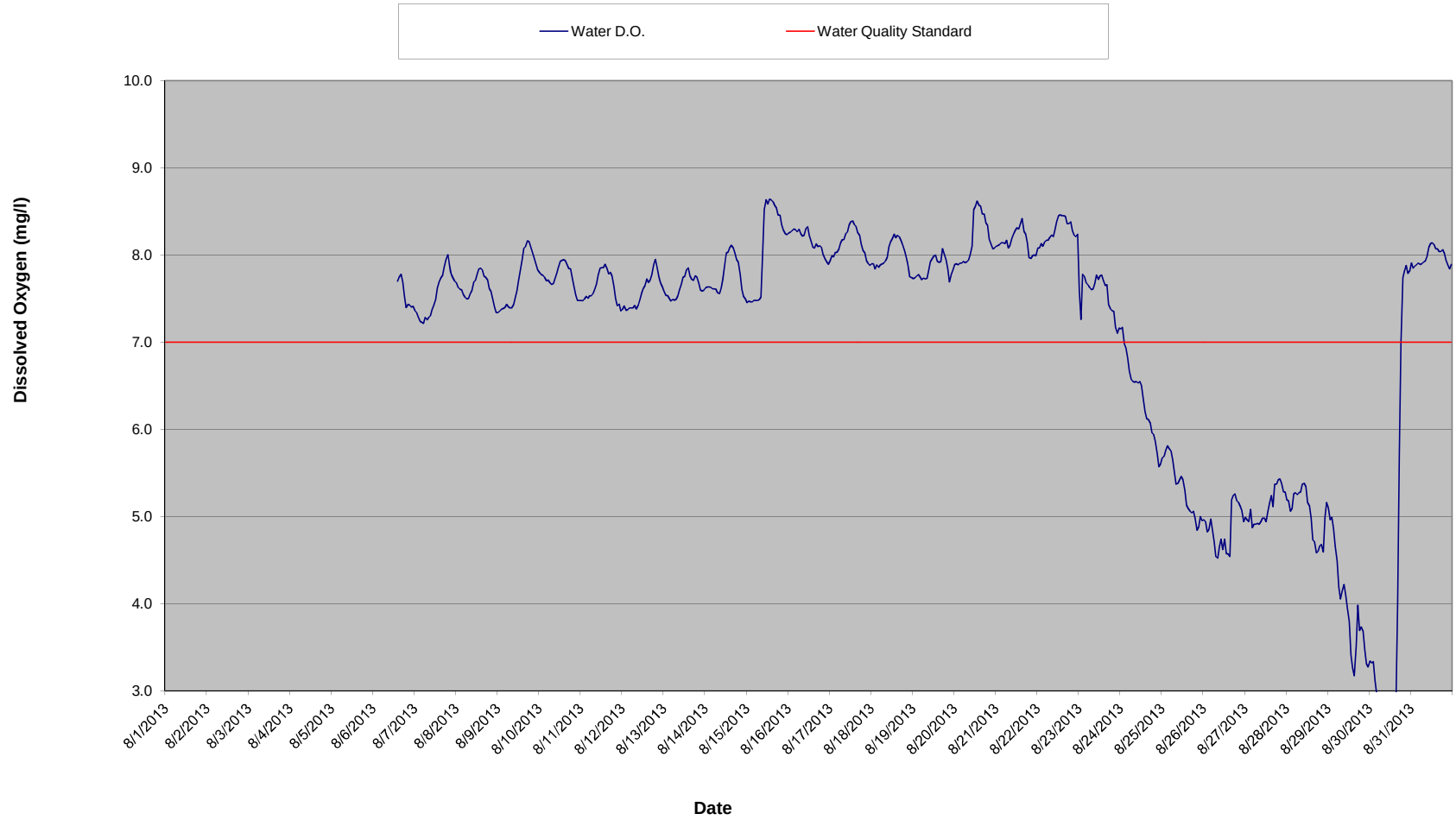
Hoist Powerhouse Dissolved Oxygen Summary - August 2013
