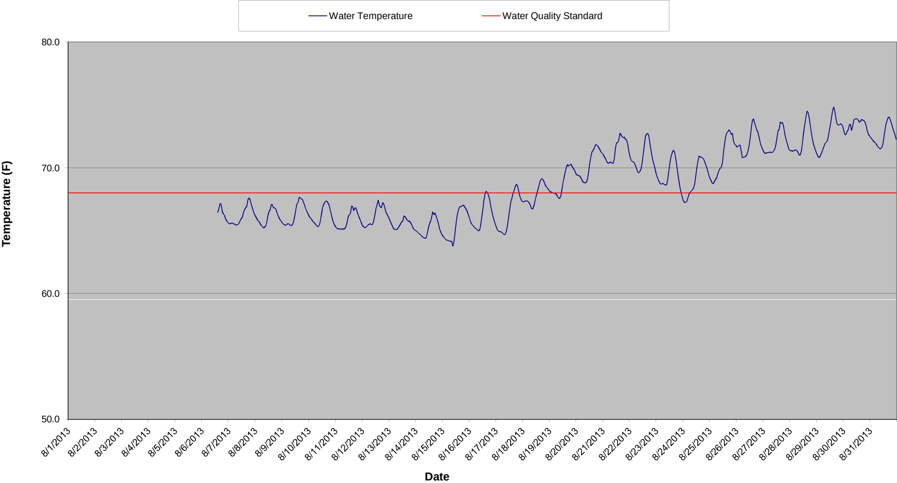
Hoist Powerhouse Temperature Summary - August 2013
