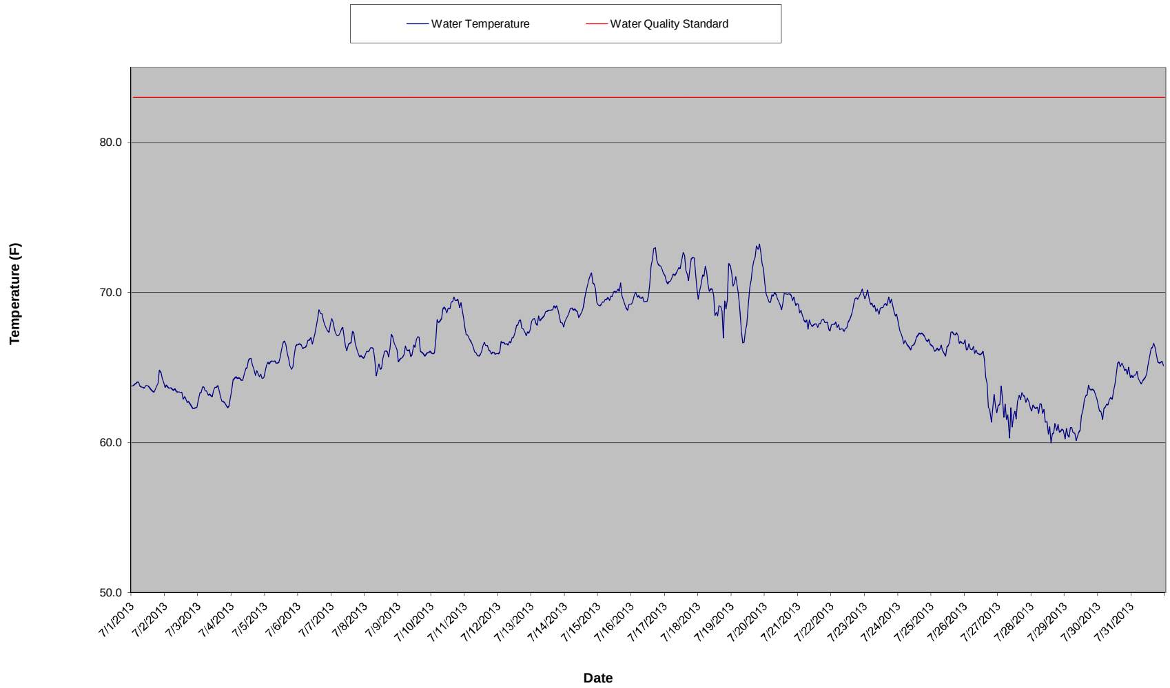
McClure Powerhouse Tailrace Temperature Summary - July 2013
