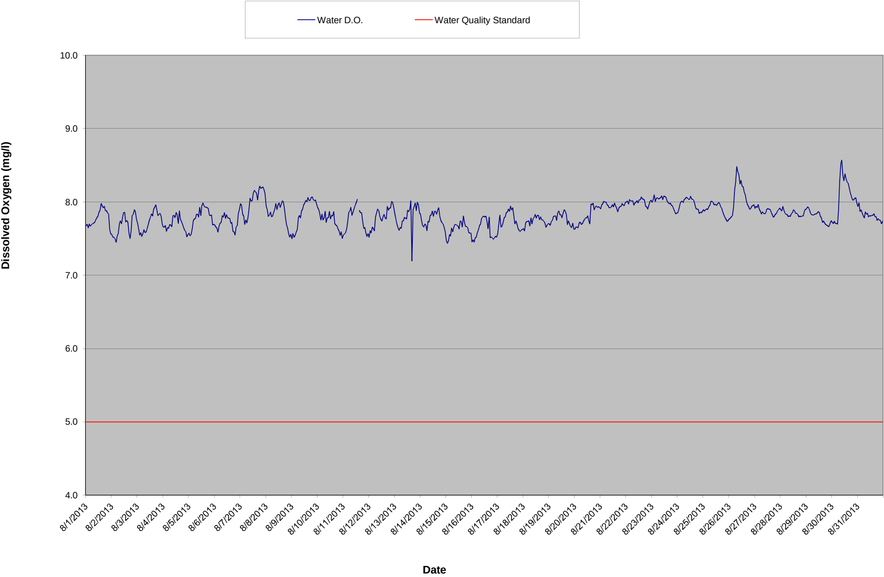
McClure Powerhouse Tailrace DO Summary - August 2013
