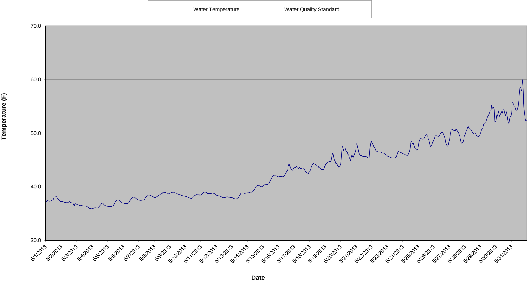
Dead River Below McClure Dam Temperature Summary - May 2013
