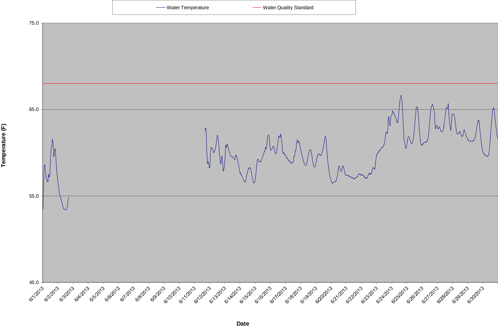
Dead River Below McClure Dam Temperature - June 2013
