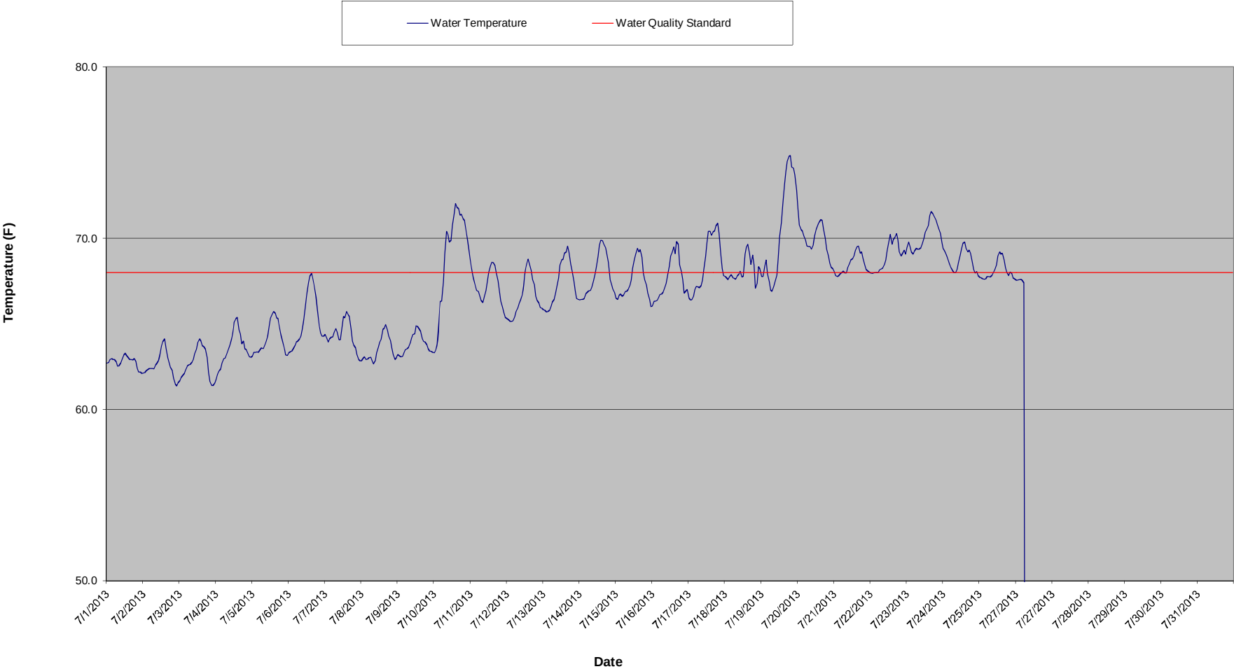
Hoist Powerhouse Temperature Summary - July 2013
