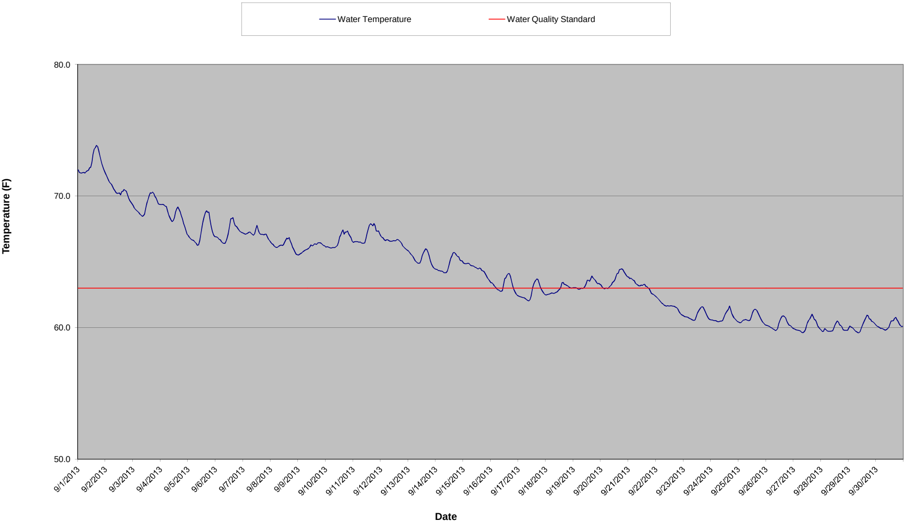
Hoist Powerhouse Temperature Summary - September 2013
