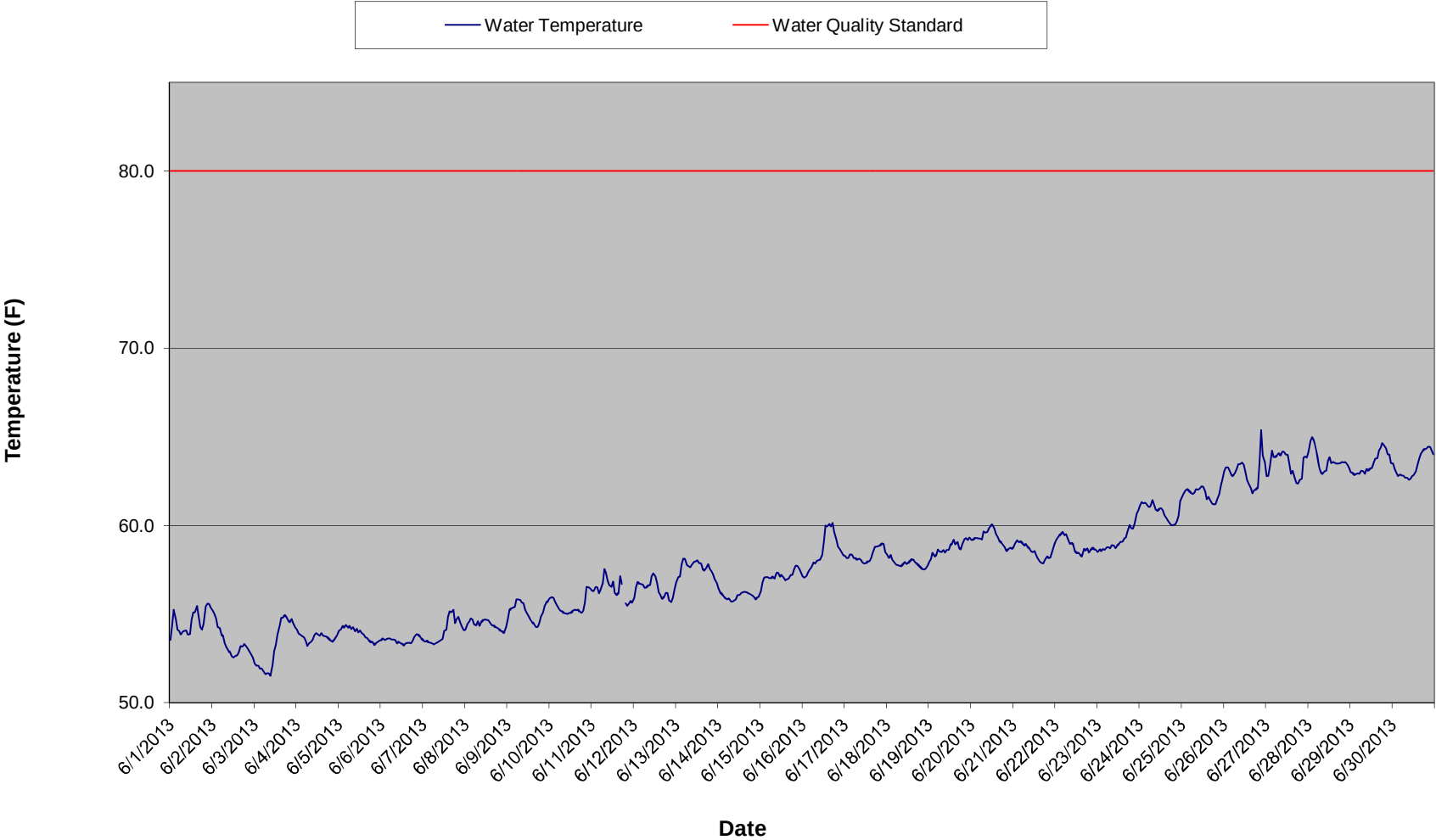
McClure Powerhouse Tailrace Temperature Summary - June 2013
