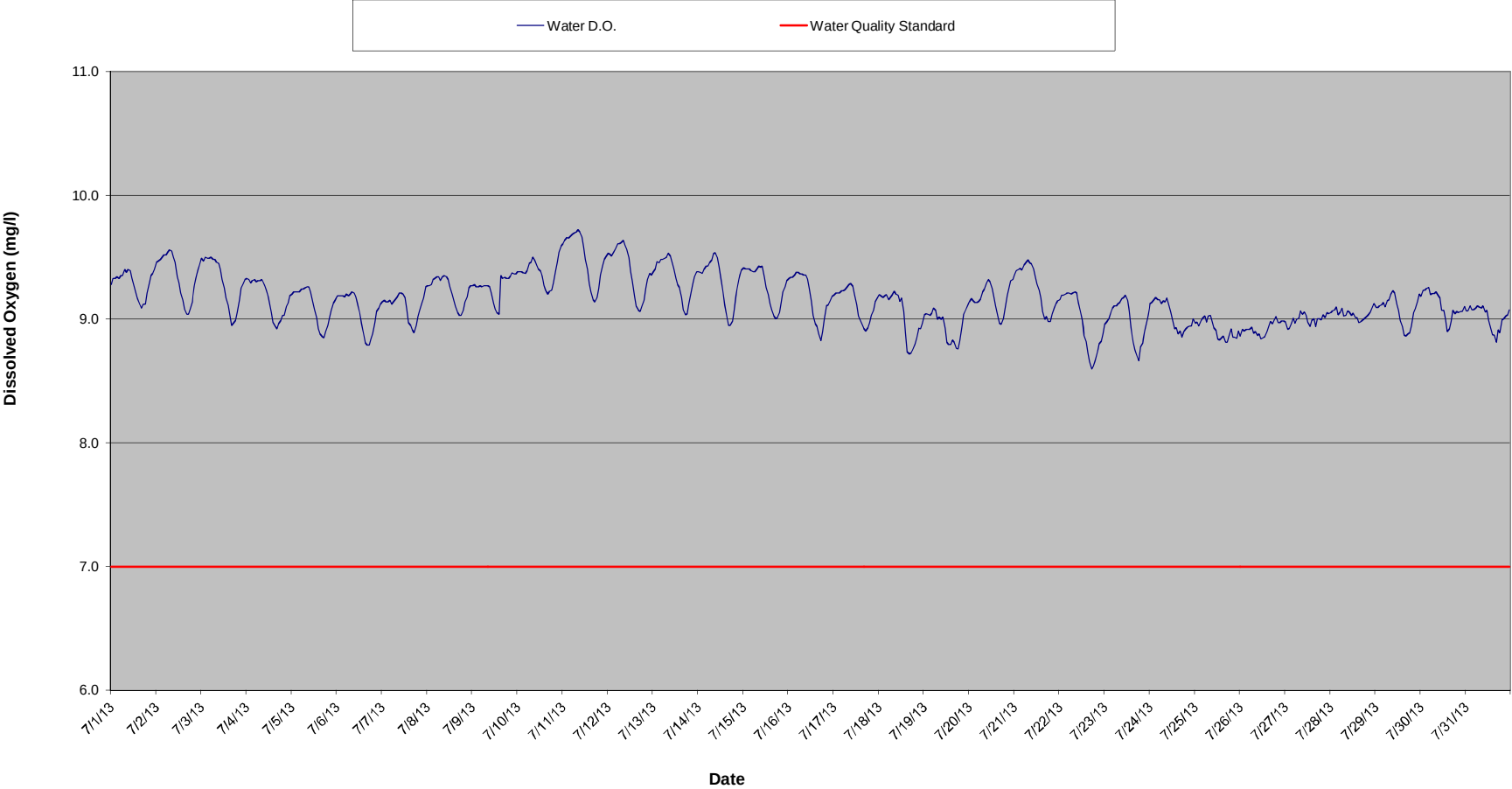
Dead River Below McClure Dam Dissolved Oxygen Summary - July 2013
