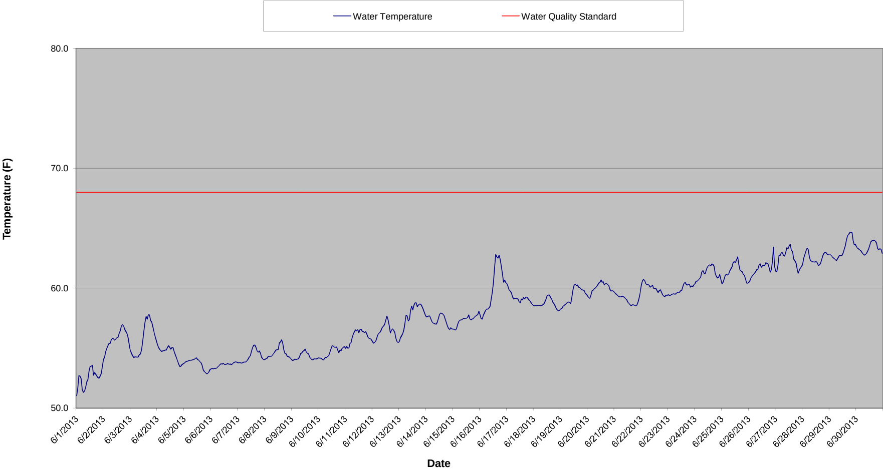
Hoist Powerhouse Temperature Summary - June 2013
