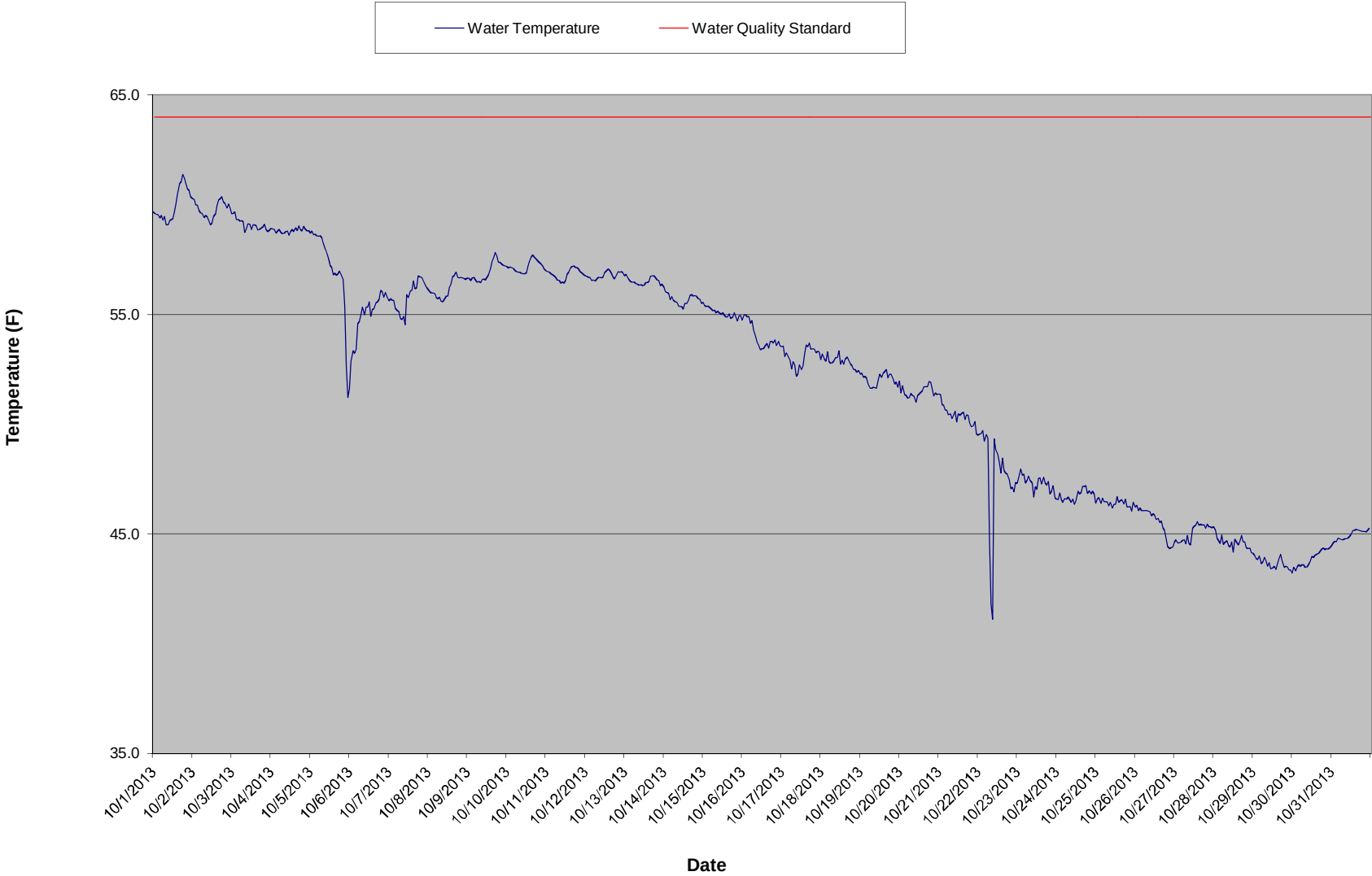
McClure Powerhouse Tailrace Temperature Summary - October 2013
