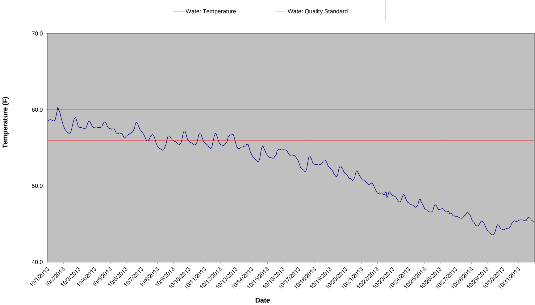
Dead River Below McClure Dam Temperature - October 2013
