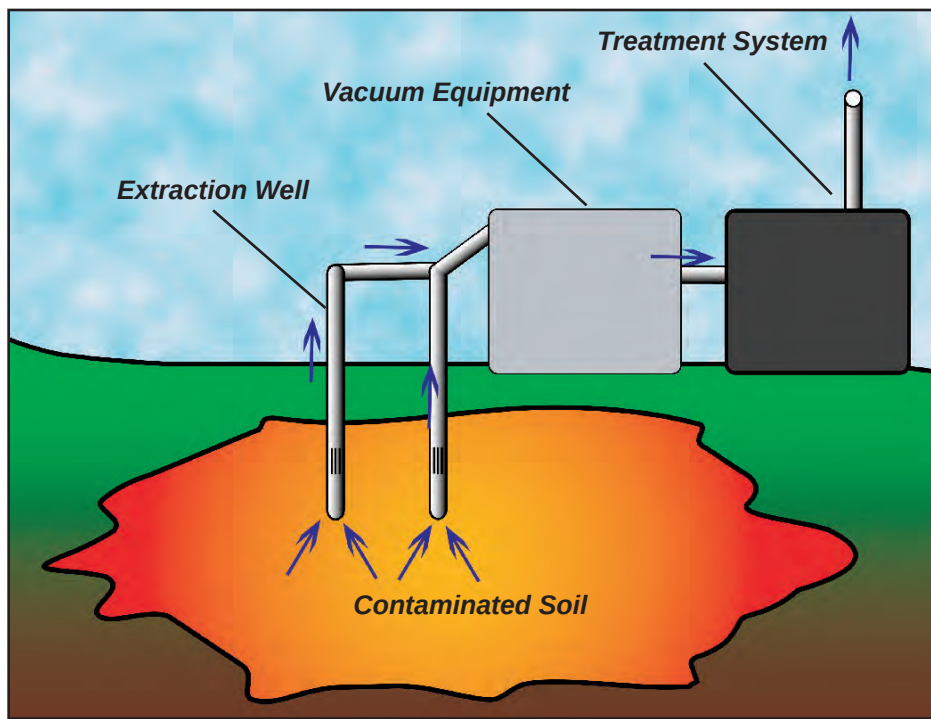
A conceptual model of a soil vapor extraction system.
