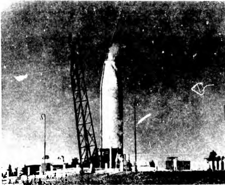
Atlas E - Dual Propellant Loading exercise - June 1961 (General Dynamics photo)
